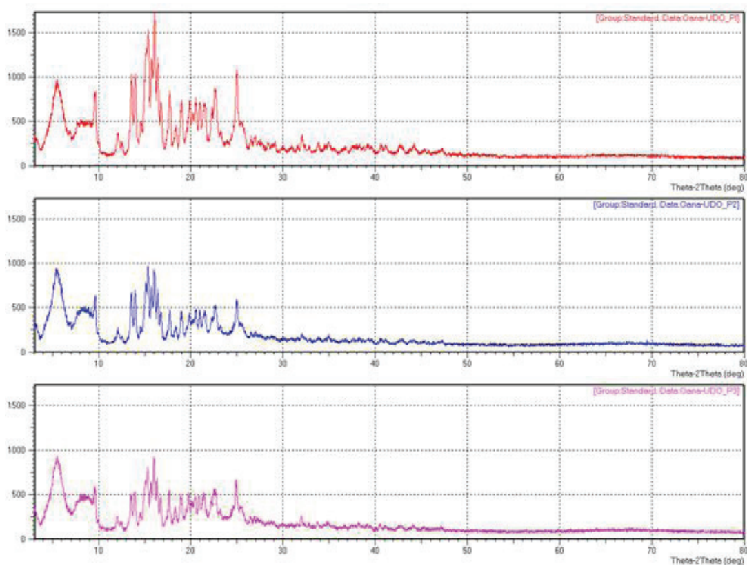
Fig. 4. XRD patterns of the three ursodeoxycholic acid samples UDO P1, UDO P2, UDO P3 (from top to bottom)
